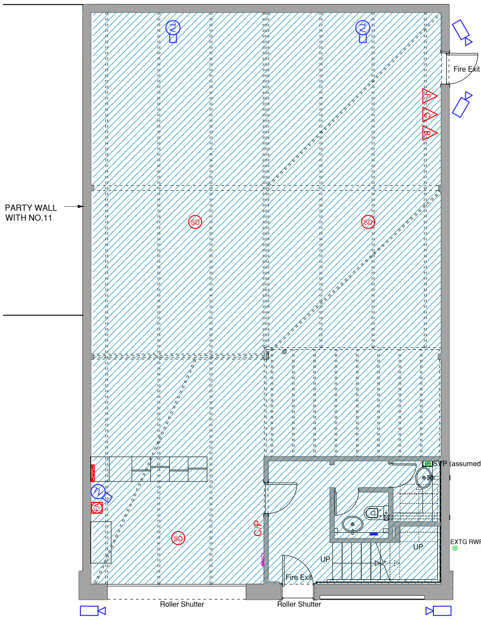
PROPOSED GROUND FLOOR PLAN TOTAL AREA 142m 2
